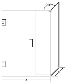
GW-1631 Corner Enclosure with Wall Channel and Corner Clip
