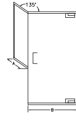
GAP-1669 2/3-B Two-Thirds Neo-Angle with Buttress Return and Header
