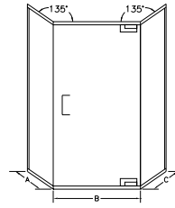
GAP-1669 Neo-Angle with Header
