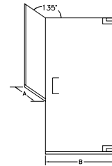
GAPW-1669 2/3-B Two-Thirds Neo-Angle with Buttruss Return
