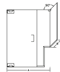
GWP-1631-NB Corner Enclosure with Buttress Return, Wall Channel & Corner Clip
