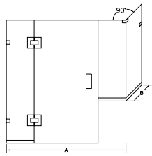
GG-1632 -B Corner Enclosure with Top Mount Corner Clip & Stationary Wall Clips
