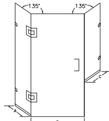
GG-1669-B Neo-Angle with Buttress Panel
