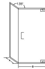
GAP-1669 2/3 Two-Thirds Neo-Angle with Header
