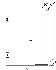
GW-1631-NB Corner Enclosure with Wall Channel and Top Mount Corner Clip
