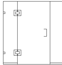
GG-1628 Panel, Door, Panel Open Above with Wall Clips
