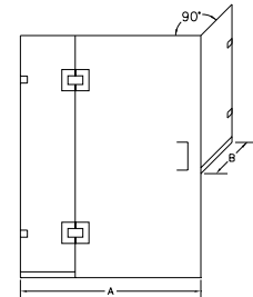
GG-1631-B Corner Enclosure with Buttruss Return, Full Height Panels
