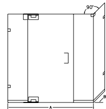
GGP-1632 Corner Enclosure Open Above with Corner and Wall Clips
