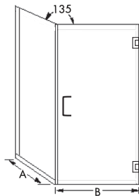
GW-1669-2/3 Two-Thirds Neo-Angle with Wall Channel
