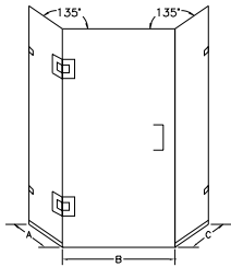
GG-1669 Neo-Angle with Header
