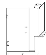
GWP-1631-NB Corner Enclosure with Buttress Return, Wall Channel & Corner Clip
