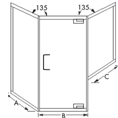
GP-1669-B Neo-Angle with Buttress Panel and Header
