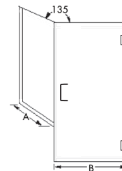
GW-1669-2/3-B Two-Thirds Neo-Angle with Buttress Panel and Wall Channel
