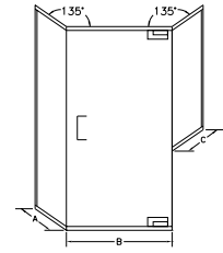
GAP-1669-B Neo-Angle with Buttress Panel & Header
