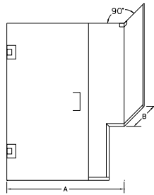
GW-1631-NB Corner Enclosure with Buttress Return, Wall Channel & Corner Clip
