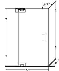
GGP-1631 Corner Enclosure Open Above with Wall Clips
