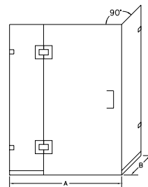
GG-1631 Corner Enclosure Open Above with Wall Clips
