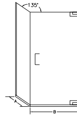
GAPW-1669 2/3 Two-Thirds Neo-Angle
