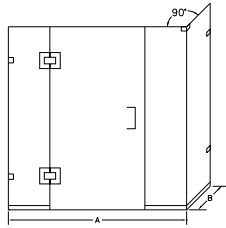
GG-1632 Corner Enclosure with Top Mount Corner Clip & Stationary Wall Clips
