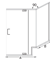
GP-1631-NB Corner Enclosure with Buttress Return and Header
