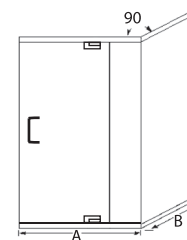
GP-1631 Corner Enclosure with Header
