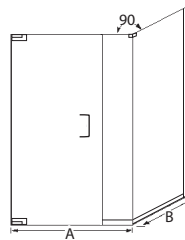
GPW-1631 Corner Enclosure without Header, with Top Mount Corner Clip
