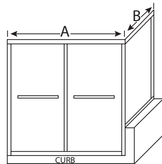
G-CS-1648-B Corner Shower Stall Enclosure with Buttress Return
