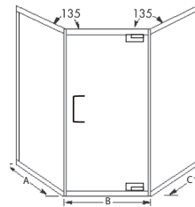
GP-1669 Neo-Angle with Header
