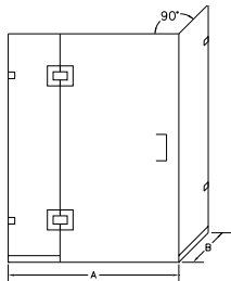
GG-1631 Corner Enclosure Open Above with Wall Clips
