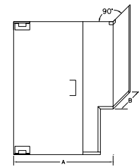
GWP-1631-NB Corner Enclosure with Wall Channel and Corner Clip
