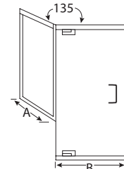
GP-1669 2/3-B Two-Thirds Neo-Angle with Buttress Return and Header
