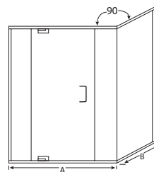
GP-1632 Panel, Door, Panel Corner Enclosure with Header
