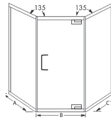
GP-1669 Neo-Angle with Header
