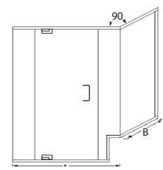
GP-1632-NB Panel, Door, Panel Corner Enclosure with Buttress Return and Header
