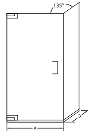
GPW-1669 2/3 Two-Thirds Neo-Angle
