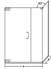
GAPW-1631-NB Corner Enclosure with Buttruss Return, without Header, with top mount corner clip
