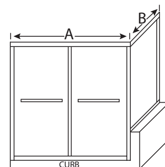
G-CS-1648-B Corner Shower Stall Enclosure with Buttress Return * Return panel is 3/8" glass
